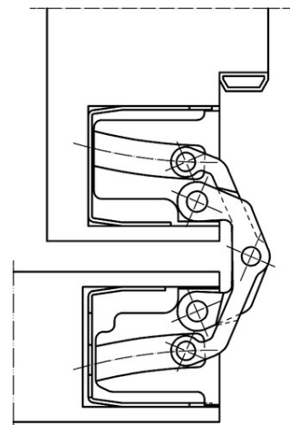
block frame 180°
