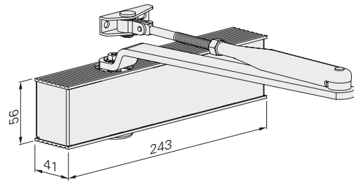
Dimensions: ECO TS-20
